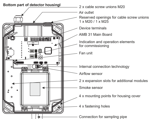
Fig. 2 Inside view of the SEC-ASD 531
